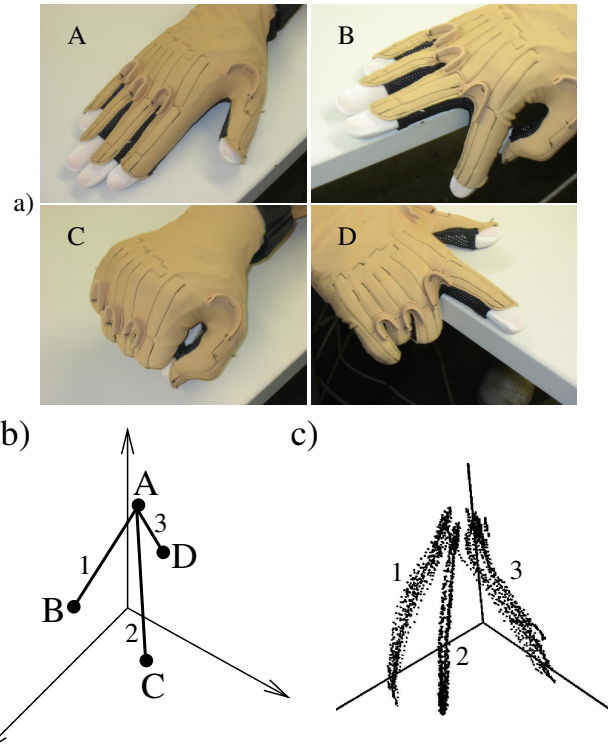
Figure 5. Structure of the grabbed trajectories for the zero isosurface of the right hand index-middle abduction. a) endpositions of the trajectories b) a sketch of the expectations about the behaviour of an abduction sensor (see text) with the endpositions shown c) real grabbed data (1 - only the index finger flexed, 2 - both index and middle fingers flexed, 3 - only the middle finger flexed)
