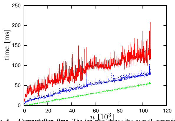
Fig. 5. Computation time. The top plot shows the overall computation time per step over the number of features. The two bottom plots divide this time, bottom to top, into downward estimation (mainly backsubstitution), bookkeeping, and upward update (mainly QR-decomposition).
