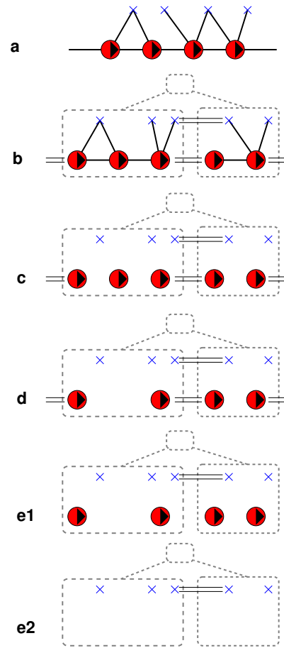
Fig. 3. Different levels of approximation. a) original nonlinear observations b) keep nonlinear observations c) linearize d) marginalize out old poses e) sparsify out old poses by first sacrificing the equality constraint and then marginalizing them out.
