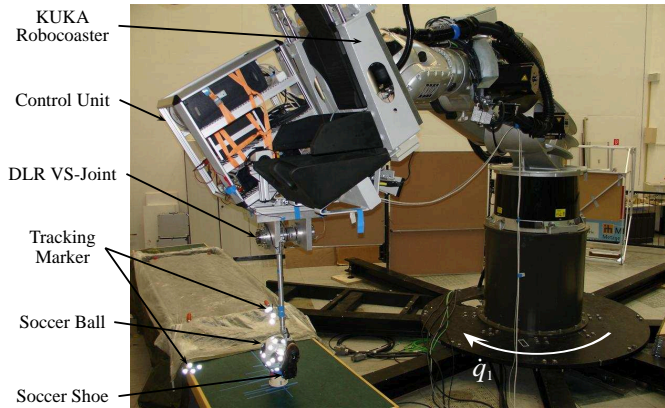
Figure 12: Test setup for hitting the VS-Joint with a soccer ball. The testbed for the VS-Joint is mounted upside down on a KUKA KR500/Robocoaster. The entire joint testbed is moved horizontally with a constant Cartesian velocity of up to 3.7 m/s by the KR500. The link hits the resting ball in non-pretensioned state with an attached foot that is equipped with a standard soccer shoe (see Fig. 16). This allows to investigate the effect of the resting joint being hit by a ball in a controlled and reproducible environment.
