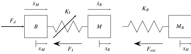
Figure 9: One-dimensional model of kicking a soccer ball with a variable stiffness robot. The robot is modelled as a mass-spring-mass system, representing the motor mass, joint stiffness, and link mass with B = 13 kg, M = 4 kg, and K_J \in \{130, 1300, 13000\} N/m. The ball is modelled as a mass-spring element with M_B = 0.45 kg, and K_{Ball} = 43.7 kN/m. B , M were selected to be the reflected inertias in case of a typical stretched out collision configuration with the DLR-LWRIII.
