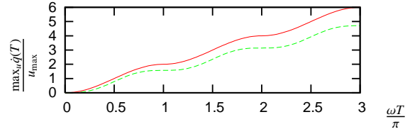
Figure 19: The speedup achievable in time T . The X-axis indicates the time \frac{\omega T}{\pi} in half-cycles of the spring-mass eigenfrequency. The Y-axis indicates the achievable joint velocity \frac{\max_q \dot{q}(T)}{u_{\max}} relative to the motor velocity. The top plot shows optimal bang-bang control, the bottom plot shows sinusoidal control.
