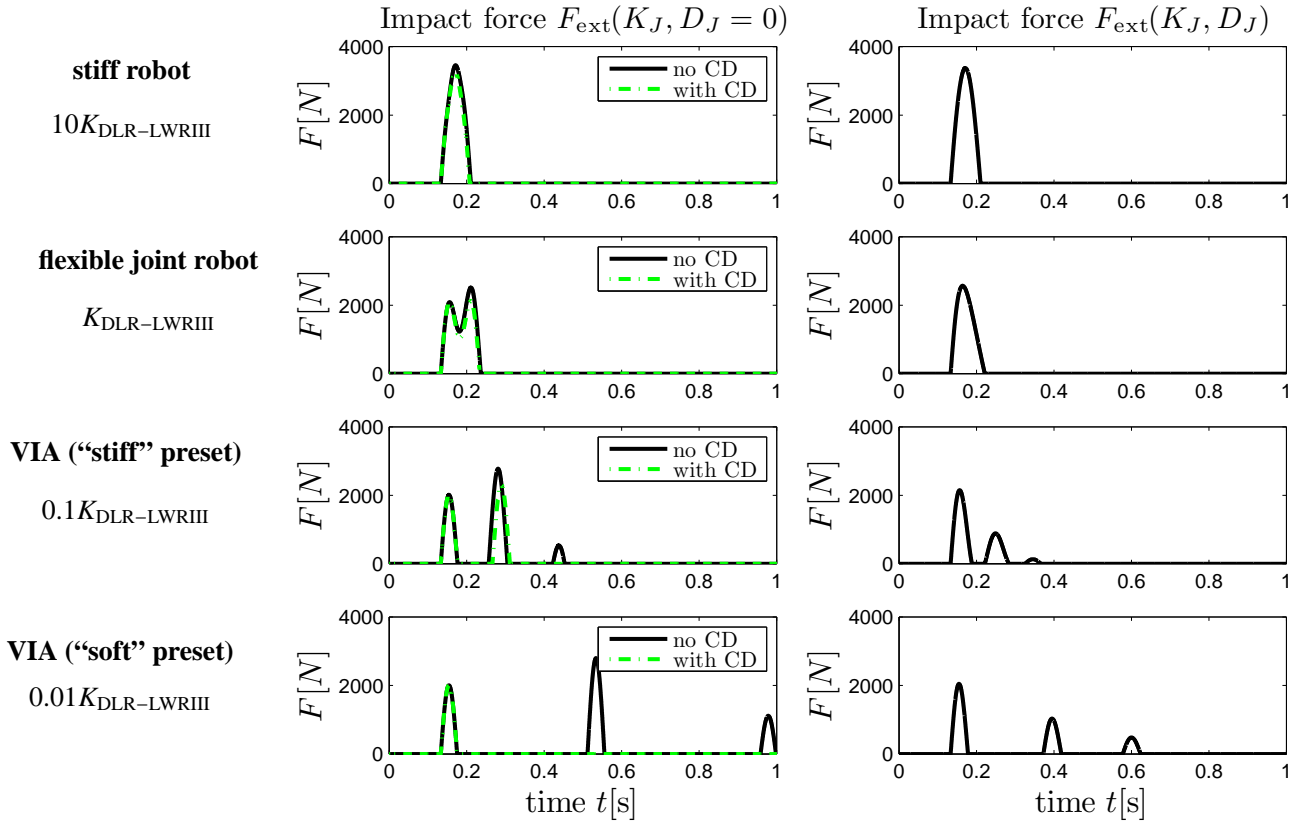
Figure 6: Impacting the abdomen at 7.5 m/s with a robot. The inertial parameters of the robot are the ones of the DLR-LWRIII and the joint stiffness is chosen to be 10, 1, 0.1, 0.01 times the one of the DLR-LWRIII. In other words, the compliance varies from very stiff to very compliant. The left plots show a robot without joint damping with and without collision detection (CD). If a collision is detected, the robot reacts by braking with full available motor force. The right plots show a critically damped link. For an intuitive understanding of this simulation please see the video provided at www.robotic.dlr.de/competitiveRobotics/ .
