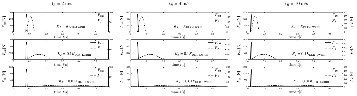
Figure 11: Simulation describing the effect of stiffness reduction on impact force and spring force for a kicking velocity of 2 m/s, 4 m/s, 10 m/s. The solid line indicates the contact force and the dashed line the spring force. The spring force decreases in magnitude and increases in duration when reducing the spring stiffness, whereas the contact force basically stays the same for each particular impact velocity. These are results from the simulation explained in Sec. 4.1.
