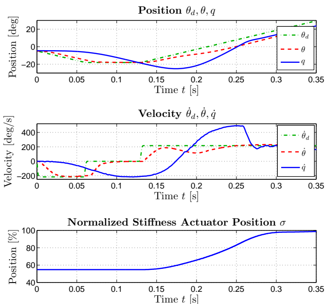
Figure 17: A strike out trajectory of the joint motor in combination with an increase of the stiffness preset are used to gain maximum link velocity.
