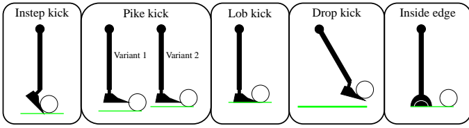
Figure 15: Kicking techniques investigated in the framework of this paper. Only the drop kick allows a foot position below the ball.
