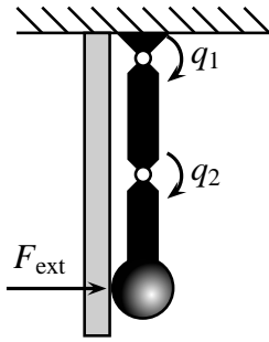
Figure 2: Example for a robot impact: A two-joint robot with joint angles q_1 = q_2 = 0 deg hits a wall with an extra mass at the TCP. The robot is decelerated by the contact force F_{ext} imposed by the wall.
