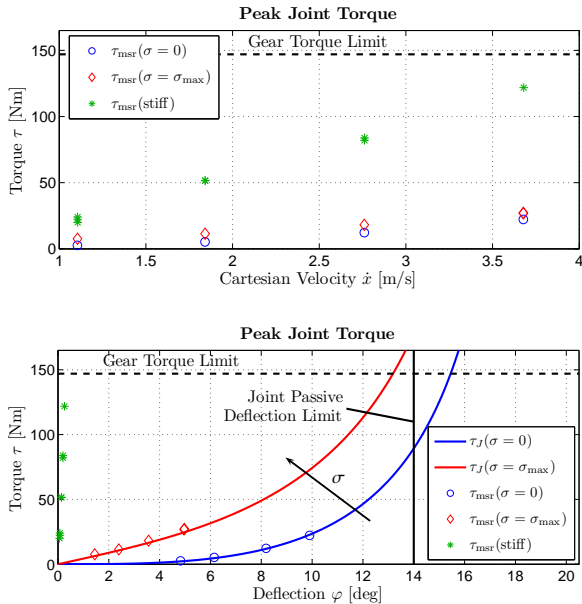
Figure 13: Top : Peak joint torque during impacts with a soccer ball and the VS-Joint. The impact velocity ranges up to the maximum velocity of the KR500/Robocoaster. Three different stiffness setups are examined: VS-Joint at low stiffness preset, VS-Joint at high stiffness preset, and an extremely stiff joint without deliberate elasticity. Bottom : Peak joint torque during impacts of a soccer ball on the soccer foot mounted on the joint. Higher impact velocities result in larger peak torque and passive joint deflection. At the same speed a soft joint stiffness preset ( \sigma = 0 ) causes significantly lower joint torque but higher joint deflection. Therefore, a very soft joint faces a higher risk of running into the deflection limits. For a very stiff joint, the gear torque limit poses an upper bound for the maximum impact velocity. Maximal two trials were carried out for each velocity and stiffness configuration.
