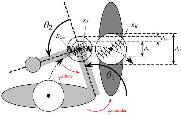
Figure 7: Two-dimensional modelling of an elbow check. The left player hits the right player with his elbow on the head. The elbow is adjusted such that it produces the worst-case impact force for each setting. View from above.
