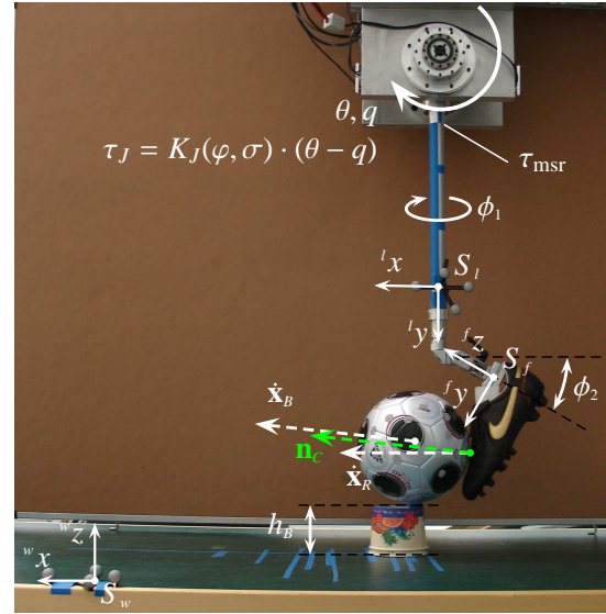
Figure 16: Test setup for kicking a ball depicted for an instep kick. The testbed for the DLR VS-Joint is mounted upside down. The angle \phi_2 between the foot and the limb (joint lever) is altered by a hinge. The height of the ball h_B is adjusted by the number of piled cups underneath and adjusted according to the investigated kicking technique (see Fig. 15). The normal on the contact point between foot and ball is denoted as \mathbf{n}_C .
