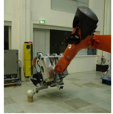
Figure 14: Left : Kicking a soccer ball at high impact speed. Right : A football kick with a KUKA KR500 weighing 2500 kg at maximum velocity. The reflected inertia during such an impact is 1870 kg.
