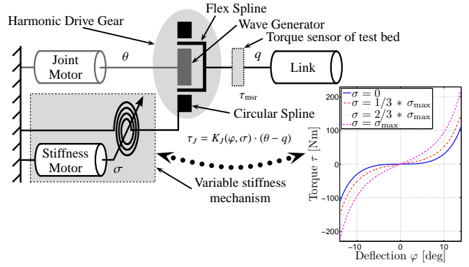
Figure 10: Principle of variable stiffness joint mechanics. The circular spline of the harmonic drive gear is supported by the VS-Joint mechanism.
