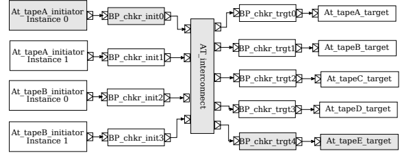
Fig. 3. Architecture of the AT-example .
