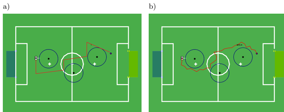
Fig. 2. Paths resulting from different approaches for obstacle avoidance: a) The previously used reactive behavior and b) the RRT planning algorithm.
