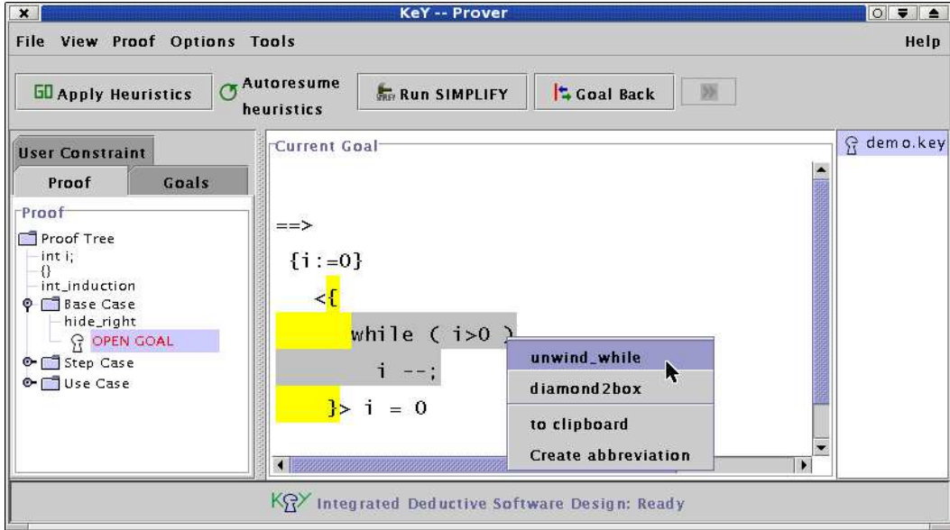
Fig. 2. Choosing a taclet to apply
