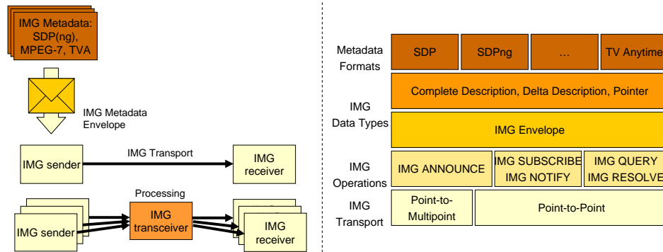
Figure 1: Architecture Overview
