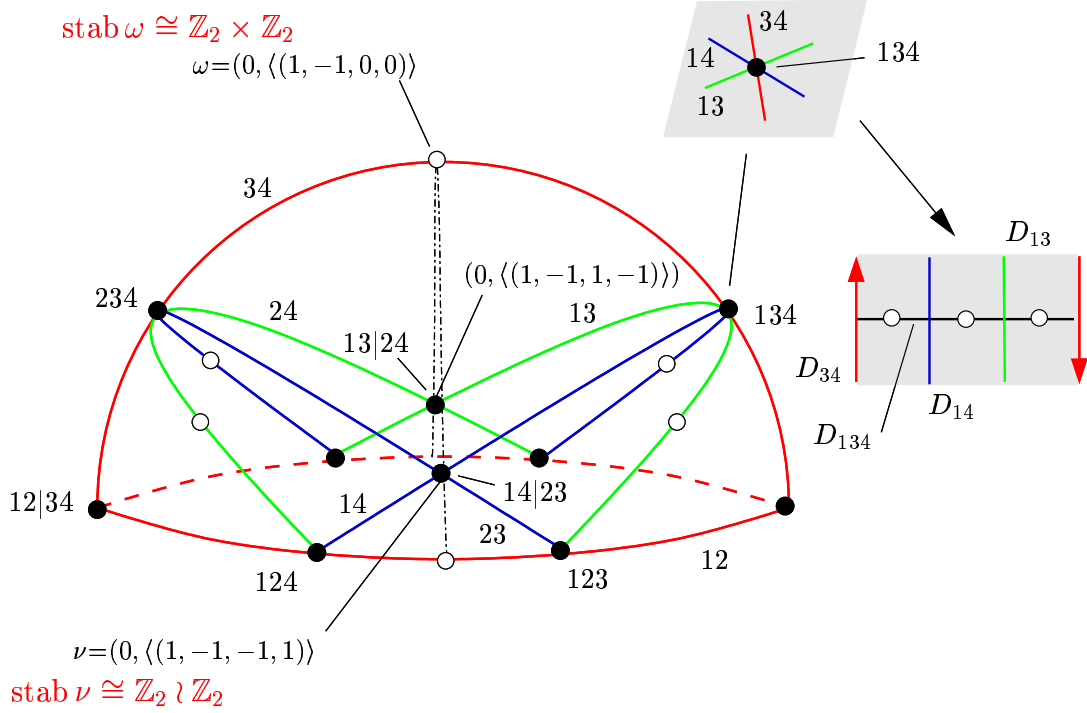
FIGURE 12. \mathfrak{S}_4 acting on \text{Bl}_{\{0\}}V , V = \mathbb{R}^4/\Delta .
