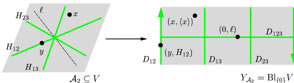
FIGURE 2. The maximal wonderful model for \mathcal{A}_2 .
