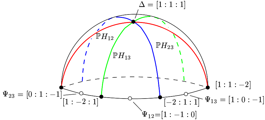
FIGURE 13. \mathfrak{S}_3 acting on \mathbb{R}\mathbb{P}^2 : the stabilizer stratification.
