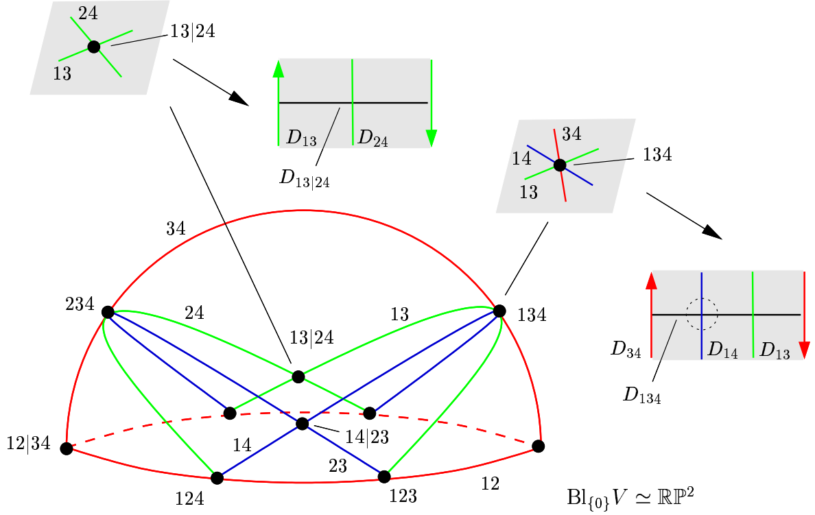
FIGURE 4. The construction of Y_{\mathcal{A}_3} .
