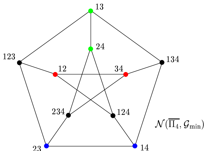
FIGURE 6. The nested set complex \mathcal{N}(\overline{\Pi_4}, \mathcal{G}_{\min}) .
