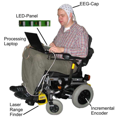
Fig. 1. A person wearing an EEG-cap and navigating the Bremen Autonomous Wheelchair Rolland . The system comprises the wheelchair's sensorial equipment, an LED-panel generating the visual stimuli, an EEG-Cap connected to a medical signal amplifier, and a processing laptop.
